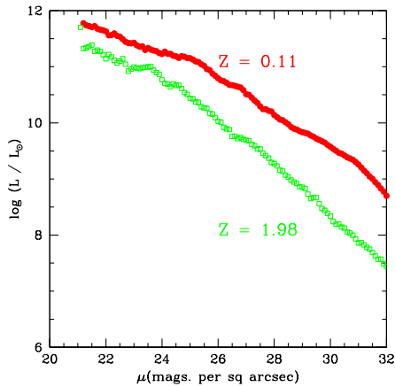
Fig. 1.3. A surface brightness histogram of all starlight from a N-body simulation by Dubinski (1998). As can be clearly seen, as the cluster evolves, more starlight is accreted (causing an offset between the two histograms), and starlight is stripped from the high-surface brightness galaxies, and re-distributed into lower surface brightness ICL features. This stripping causes the surface brightness histogram slope to become more shallow over time. This relation, which is in principle observable, may allow us to place limits on the dynamical age of galaxy clusters.
