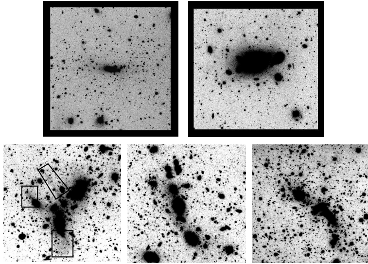
Fig. 1.1. Images of five clusters observed in this survey. From left to right and top to bottom, they are: Abell 1413, MKW 7, Abell 1914, Abell 1234, and Abell 1553. The last three clusters show only the central section of the image; these clusters show a wealth of ICL substructure. Many of the brighter galaxies at the center of each cluster lie within a low surface brightness common envelope, and there are clearly defined tidal features, most noticeably in Abell 1914 (denoted by the boxes). This in contrast to the first two clusters, which had less substructure (Feldmeier et al. 2002).
