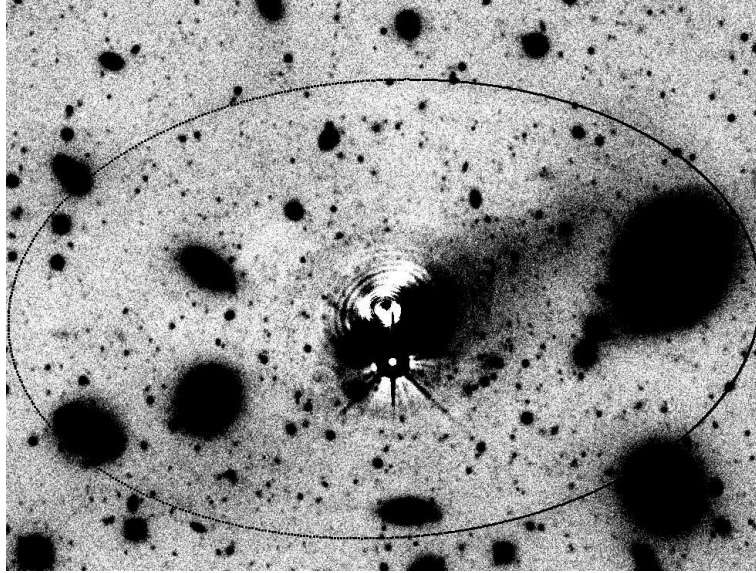
Fig. 1.2. Our residual image for MKW 7, after the best-fitting elliptical model of the cD + ICL has been subtracted. The black ellipse shows where the measured surface brightness has a signal-to-noise greater than five. A large tidal plume is apparent leading from the center of the image to the right (south), and up (west) of the galaxy’s nucleus. The magnitude of this plume is approximately equal to a small galaxy ( M_V \sim -17 )
