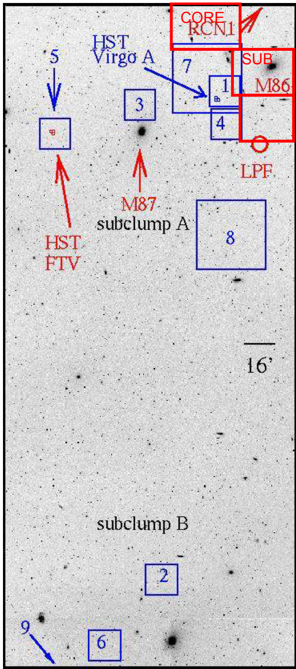
Figure 1. Images of portions of the Virgo cluster (left) and the Fornax cluster(right). The regions surveyed for IPN are shown as the boxes in each image. There are over 400 IPN candidates detected in Virgo, and over 100 detected in Fornax at the current time.
